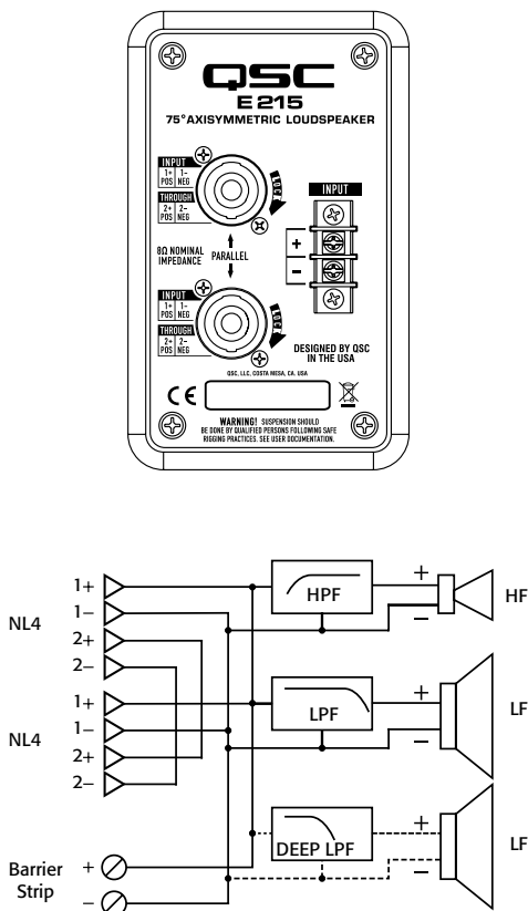
E215 Block Diagram and Input Plate
